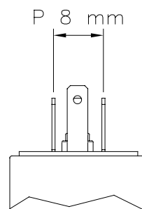
4 pin MicroDIN Form C Protection IP65
